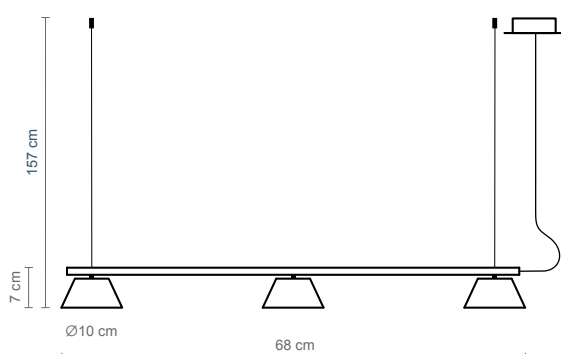
Absidiola c lineal 3 CONICA
