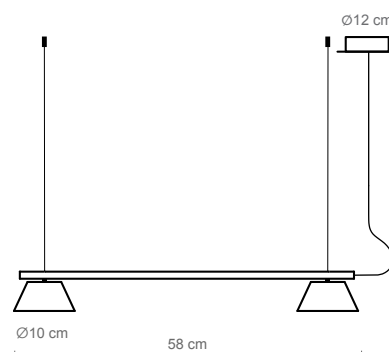
Absidiola c lineal 2 CONICA
