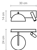
Absis a lector horizontal
