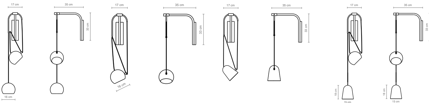
Sirius a 2 B+B
